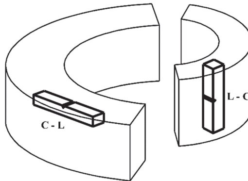
Specimen Notch Orientation
