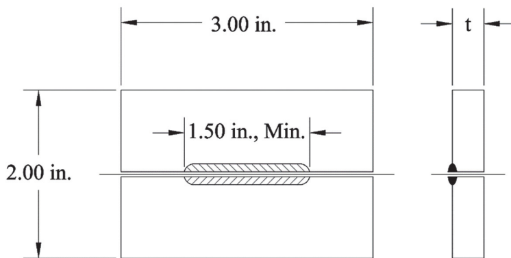
FIGURE X2-1 Longitudinal-Bead Underbead Cracking Test Specimen
