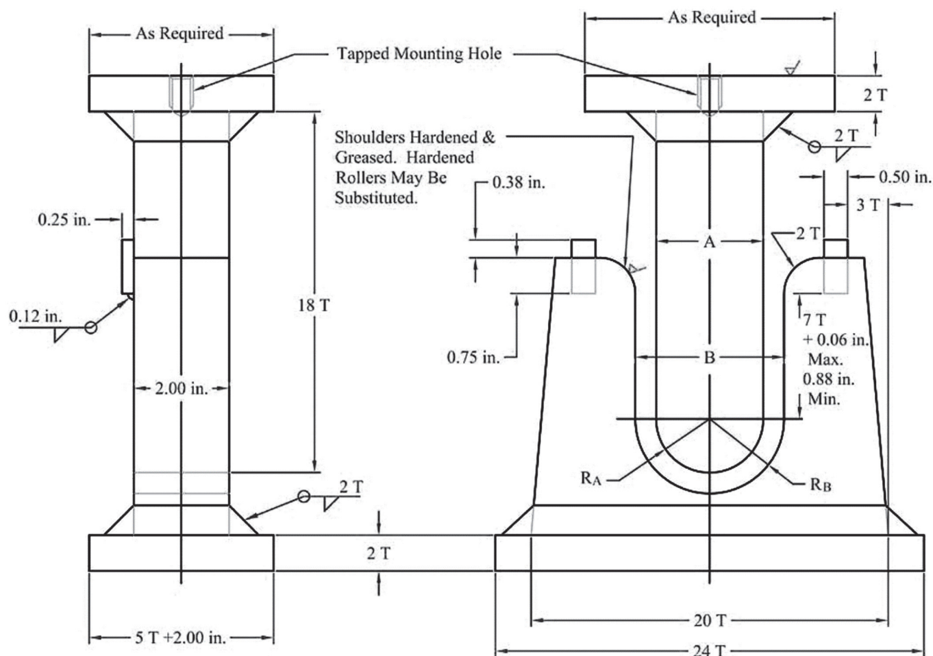
Guided-Bend Test Jig Dimensions
